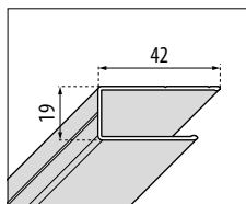
WALL A - R - F - AH - PH - FH
