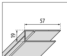
EXTENSION A - R - F - AH - PH - FH
