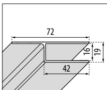
WALL side wall mounting all models
